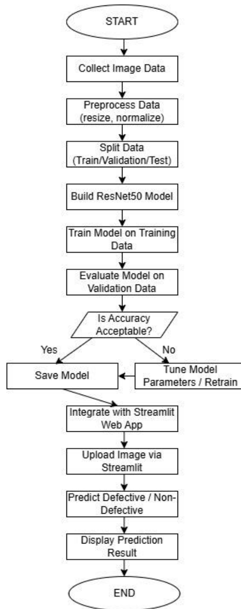
Fig 4.3.1 – Activity Diagram
