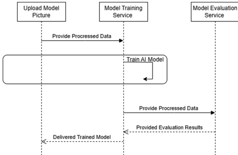
Fig 4.4.1 - Sequence diagram
